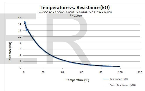
Fig.3 Resistance Vs Temperature Characterization Results
