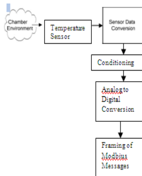
Fig.2 Slave 1 Functional Block Diagram
