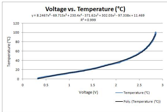
Fig.4 Temperature Vs Voltage Characterization Results
