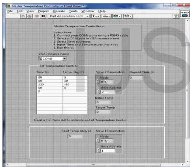
Fig.6 Master Temperature controller VI front panel
