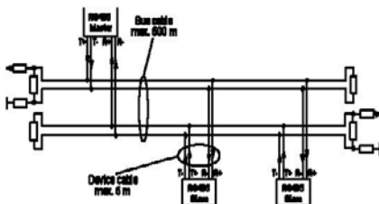
Fig.5 RS485 4-wire interface setup6
